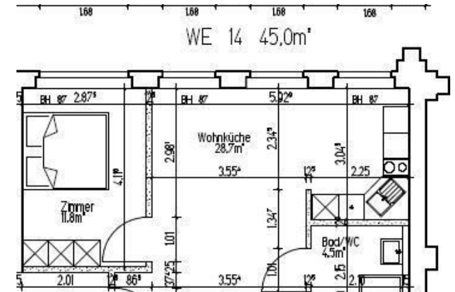
Grundriss WE 14
